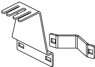
Anti-rotation bracket
